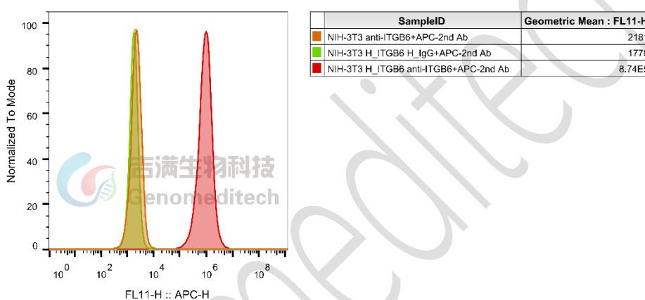
Figure 1 | H_ITGB6 NIH-3T3 Cell Line (Cat. GM-C41634) was determined by flow cytometry using Anti-ITGB6 hIgG1 Antibody(SGN-B6A) (Cat. GM-81622AB ).
